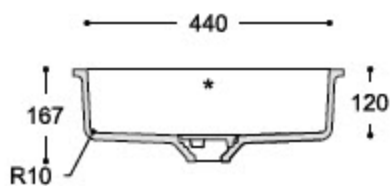
CROSS-SECTION
